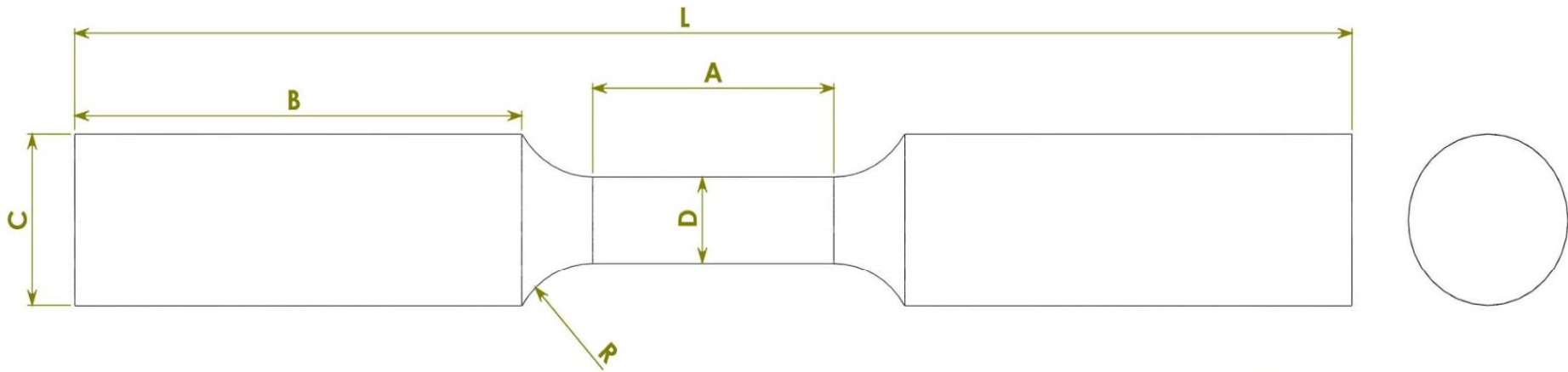
Tensile Test Specimen (Round)
